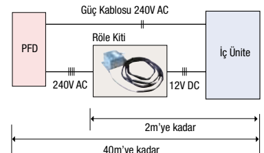
PFD4-15WR-E (opsiyonel)
